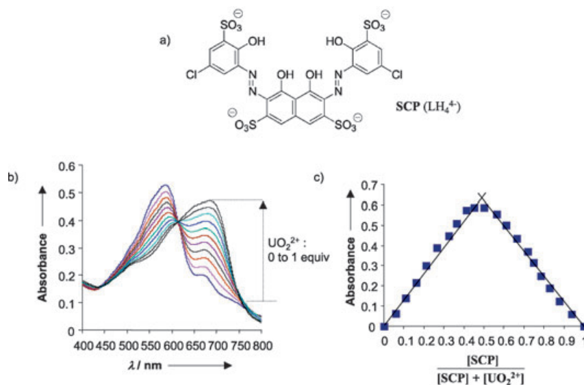
Figure 1. a) Sulfochlorophenol S ( \text{SCP} ) structure; b) UV/Vis spectra and c) Job plot of \text{SCP} and \text{SCP}/\text{UO}_2^{2+} mixtures at pH 7.4 (absorbance measured at 640 nm).
