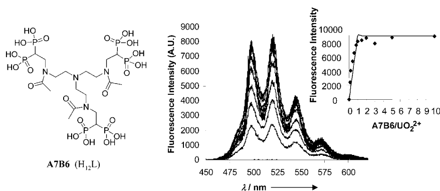
Figure 6. Structure of ligand A7B6 . Spectrofluorescence titration of a solution of \text{UO}_2^{2+} ( 4.2 \mu\text{M} ) by A7B6 in 0.1 \text{ M NaClO}_4 , pH 5.5. The inset shows the experimental and theoretical uranyl fluorescence intensity as a function of A7B6 / \text{UO}_2^{2+} ratio at \lambda_{\text{exc}} 266 \text{ nm} , \lambda_{\text{em}} 519 \text{ nm} .
