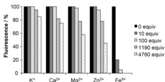
Figure 7. Selectivity of the A7B6 / \text{UO}_2 complex in the presence of metal cations. [ A7B6 / \text{UO}_2 ]=4.2 \mu\text{M} ; [ \text{NaClO}_4 ]=0.1 M; [competitive metal]=0 to 20 mM; pH 5.5
