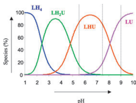
Figure 2. Thermodynamic constants and speciation diagram of SCP / \text{UO}_2^{2+} complexes calculated by using pHab [18] and HYSS [19] programs, respectively (see Experimental Section). Values in parentheses give the estimated in the least significant figure based on the variation between replicate experiments. LH 2 U : \log \beta_{112} = 37.8(1) , LHU : \log \beta_{111} = 33.0(1) , LU : \log \beta_{110} = 24.9(3) .
