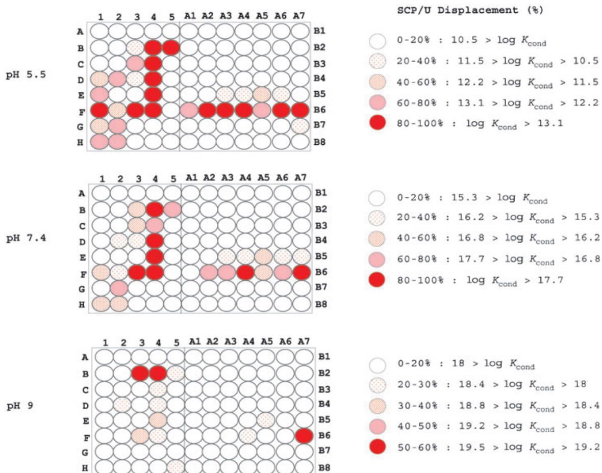
Figure 5. Screening results: Displacements (%) of the SCP/ \text{UO}_2^{2+} complex are presented in a color-coded format for clarity reason. \log K_{\text{cond}} (estimates) were calculated by using the HYSS program supposing that the complex competitive ligand/ \text{UO}_2^{2+} is 1:1. For details on the procedure, see the Experimental Section.
