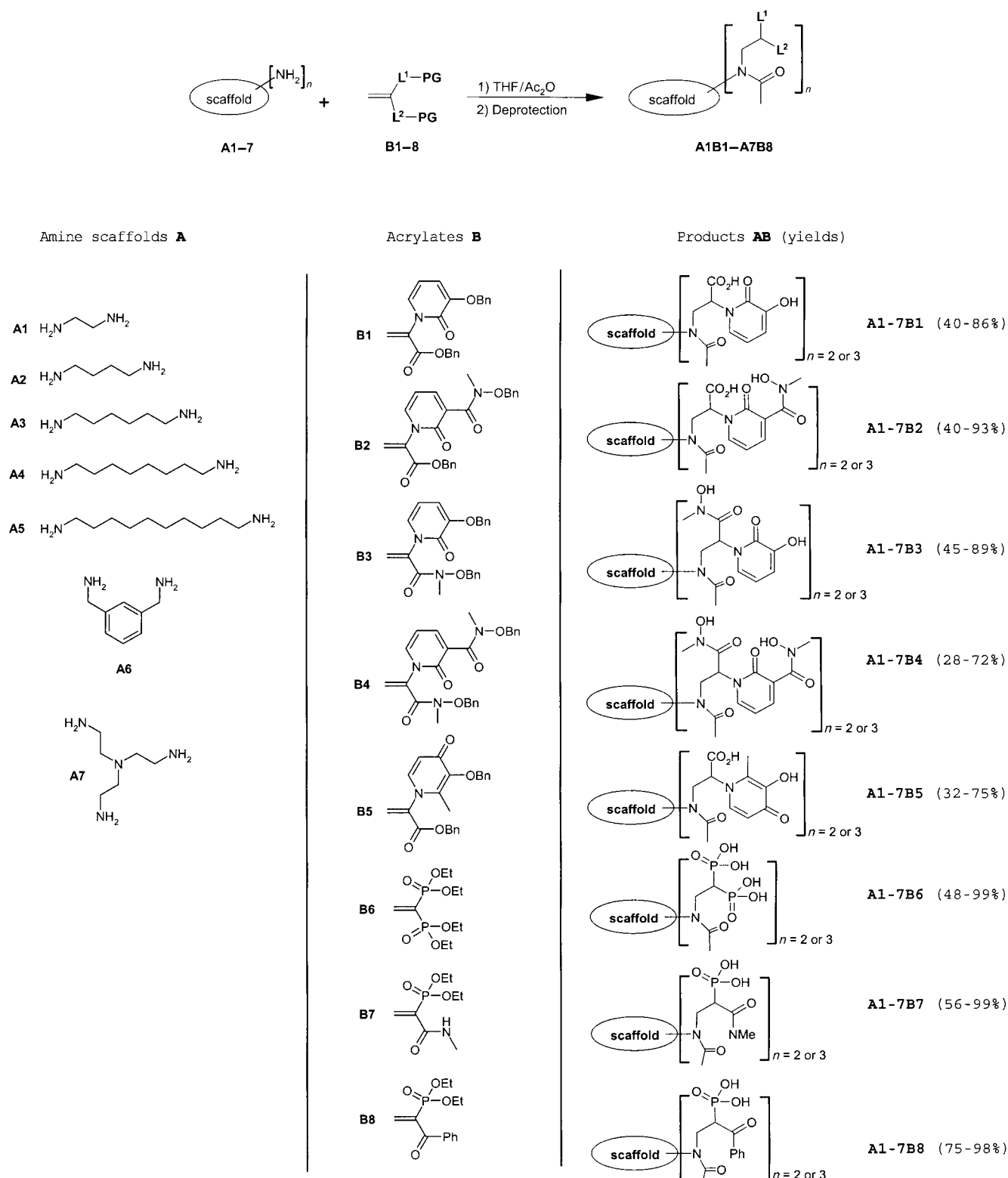
Figure 4. Parallel synthesis of ligands A1B1 to A7B8 . Michael additions were run with an excess of acrylates B in THF or DMF and then quenched by an excess of \text{Ac}_2\text{O} . Crude mixtures were then concentrated and purified through filtration on silica gel. Removal of the protective groups ( PG ) of the chelating moieties ( L 1 and L 2 ) were carried out by Pd hydrogenation or by TMSBr to afford A1-7B1-5 and A1-7B6-8 , respectively (see Experimental Section). LC-MS controls showed more than 85 % purities for each products. All compounds have been fully characterized by using ^1\text{H} , ^{31}\text{P} NMR and mass spectroscopy.
