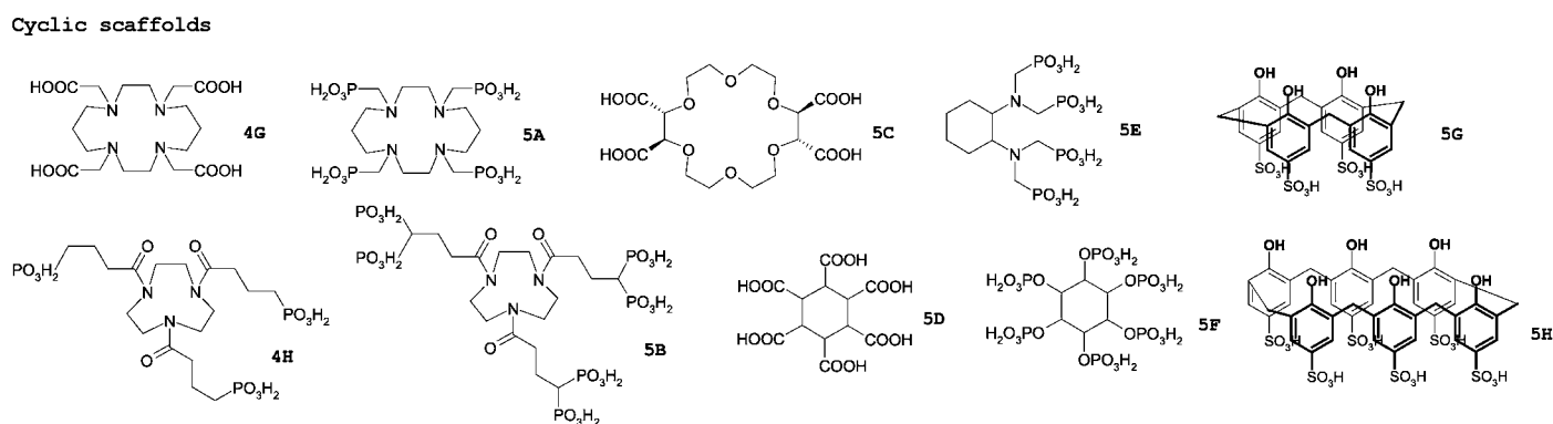
Figure 3. Ligand library.
